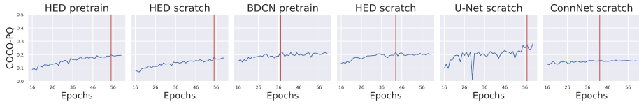
Fig. 3: COCO-PQ score of the networks under test for Stage 1 (Deep Edge Filtering), computed on the validation set, for each training epoch. The red vertical bar indicates the best model we retained to compute the results on the test set.
