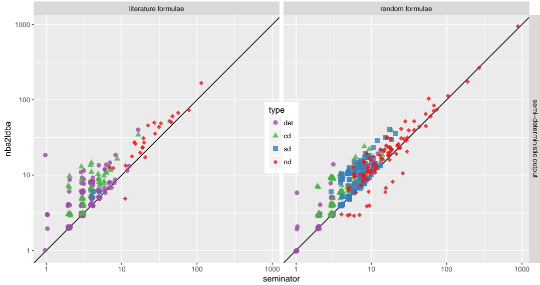
Figure 4: Comparison of the size of semi-deterministic automata produced by Seminator and nba2ldb (both without reductions) on random formulae and on formulae from literature. Scatter plots are colored according to the output type of ltl2tgba -D . Scales are logarithmic.
