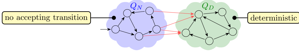
Figure 1: Structure of a semi-deterministic automaton. The green cloud is deterministic and contains all accepting transitions and states that are reachable from them. In a cut-deterministic automaton, the blue cloud is deterministic too.
