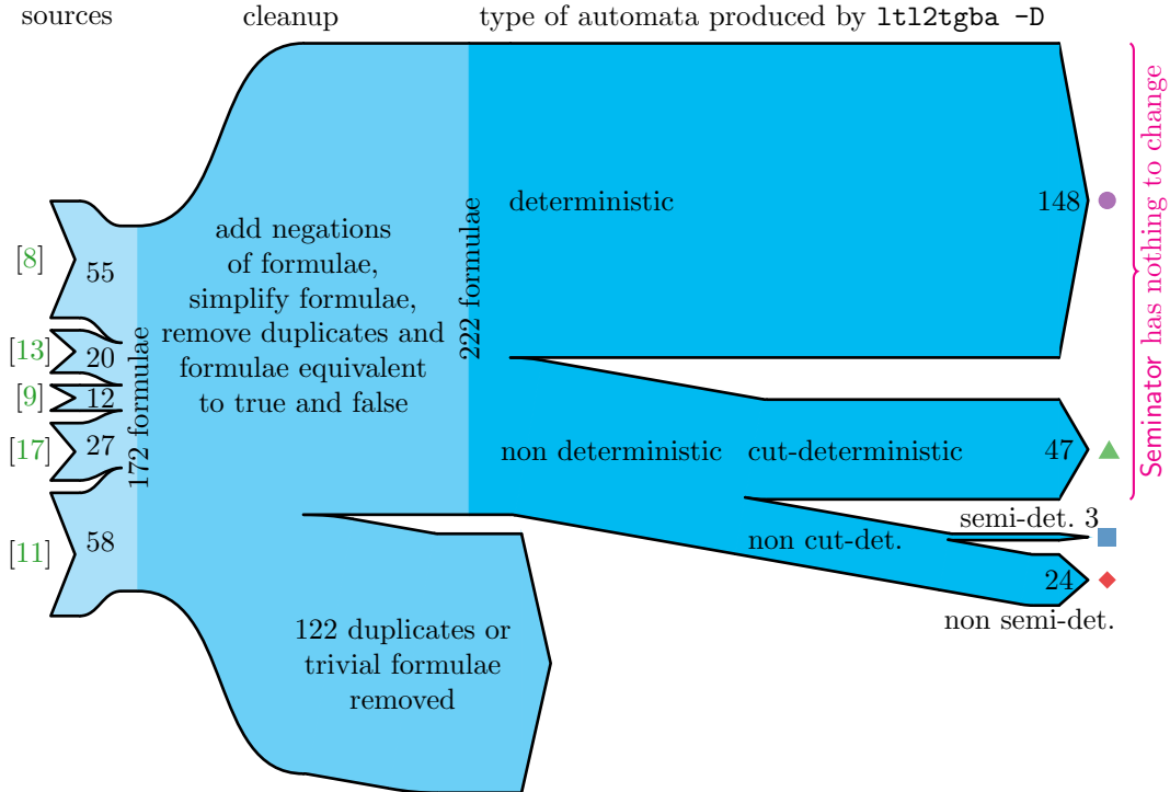
Figure 2: Preparation of the formulae from the literature, and classification according to the four types of automata produced by ltl2tgba -D .
