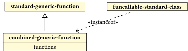
Figure 4: Combined Generic Functions
