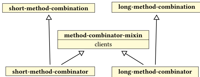
Figure 3: Method Combinator Classes Hierarchy
