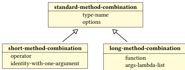
Figure 2: SBCL Method Combination Classes Hierarchy
