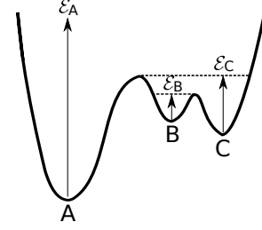
Fig. 2: Illustration of the extinction values \mathcal{E} of three minima. The order is A < C < B . B merges with C , C merges with A .
