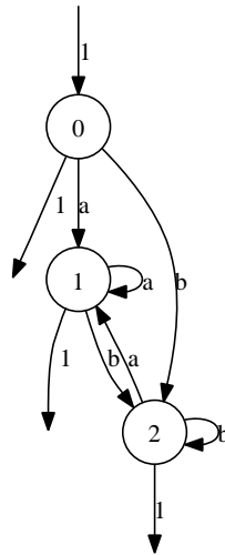
A { 3 states, 6 transitions, #I = 1, #T = 3 }
