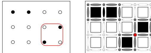
Fig. 1: From a digital set X \subseteq \mathbb{Z}^2 to its immersion \mathcal{I}(X) in \mathbb{H}^2 ; sets are depicted in black, and the boundary of \mathcal{I}(X) in \mathbb{H}^2 is in gray or red.
