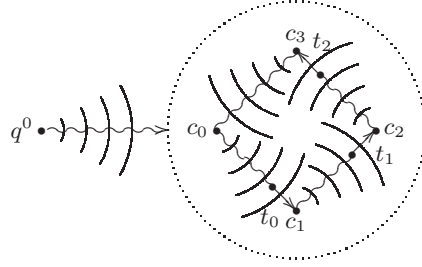
Fig. 5. Computing an accepting run for a TGBA.
