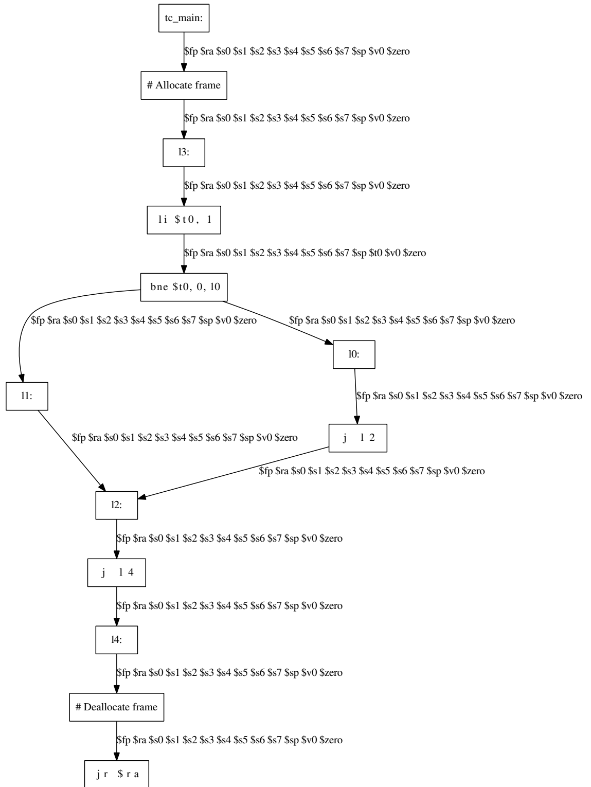
File 4.84: and.main._main.liveness.gv
