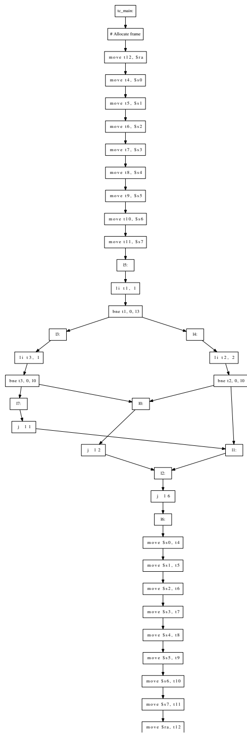
File 4.80: ors.main._main.flow.gv
